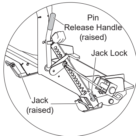
Detach HT Series™ Blade
