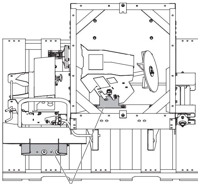
Retirer les supports.
